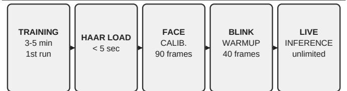
Fig. 1. Five-phase startup: Training → Haar Load → Face Calibration → Blink Warmup → Live Inference.
