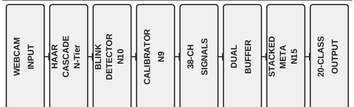
Fig. 2. System architecture: webcam → Haar cascade → blink detector → calibrator → 38-CH signals → dual buffer → stacked meta-learner → 20-class output.
